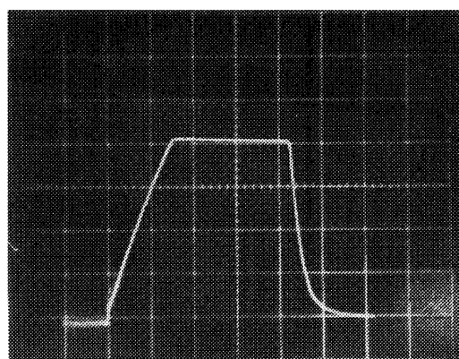
FIGURE 18A. SUPPLY TURN-ON AND TUNOFF CHARACTERISTICS
